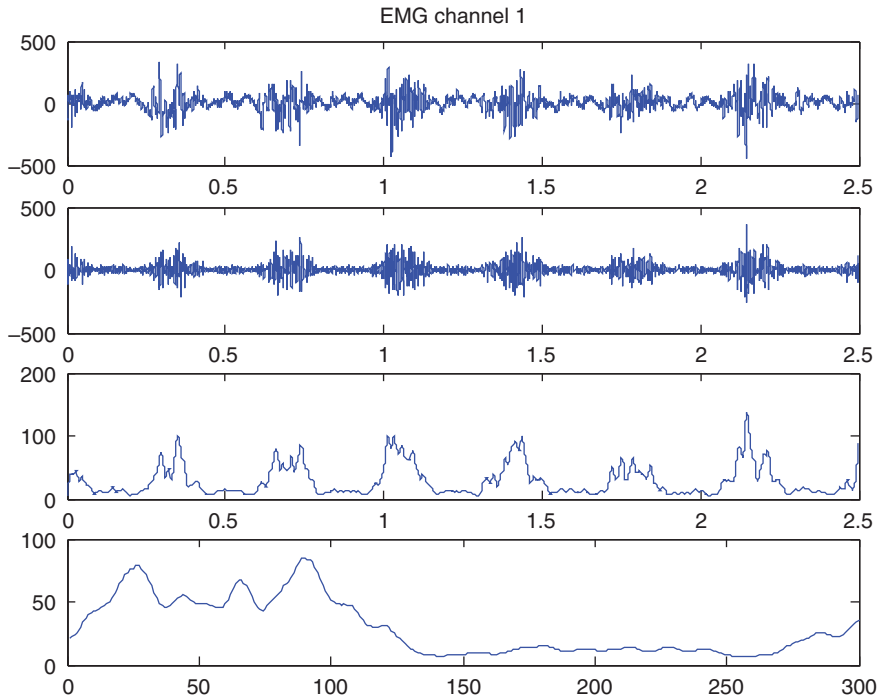
Figure 2 A typical representation of raw and smooth rectified surface EMG of baseline walking for gluteus medius muscle. Each block represents in ascending order: (1) raw EMG recording, (2) high and low pass filtered, (3) full wave rectified and smoothed, (4) one selected gait cycle of data.
